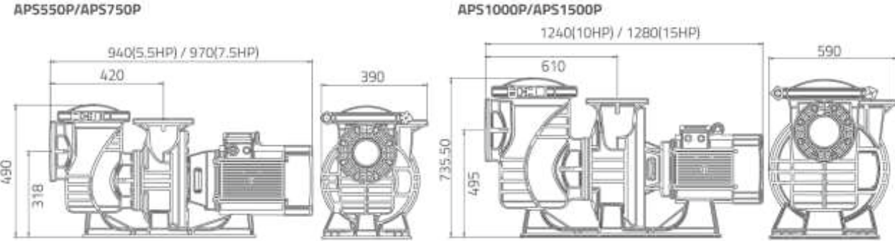
自吸泵: APS550P, APS750P 离心泵: APS1000P and APS1500P
